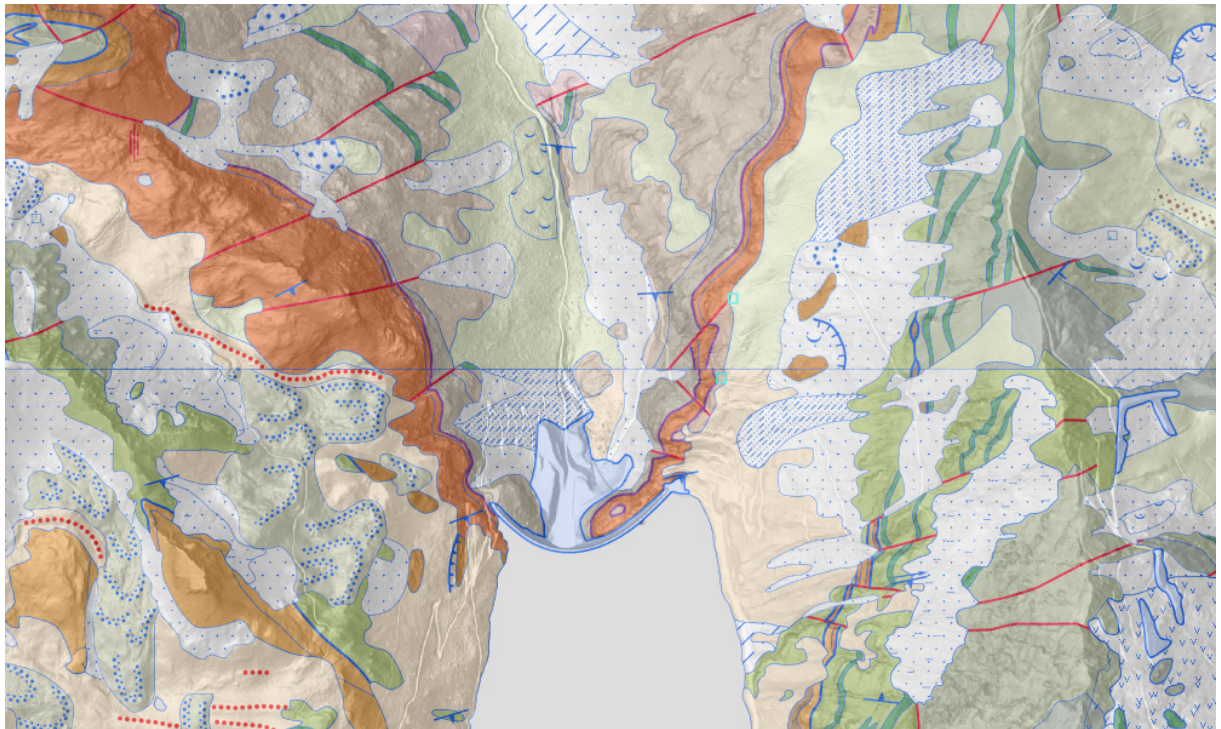
Figure 1: Extract of swissGEOCOVER2d and example of representation
